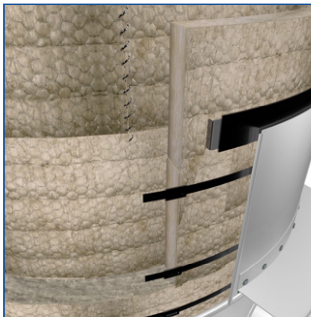
Figure 16. VERTICAL VESSEL DETAIL 1
