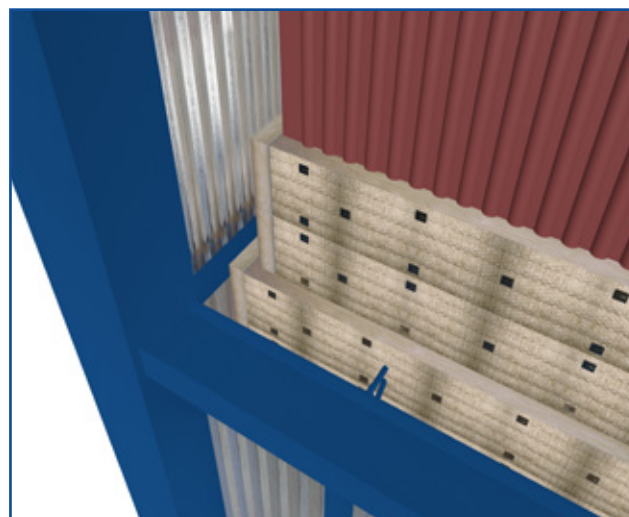
Figure 28. BOILER DETAIL 1
