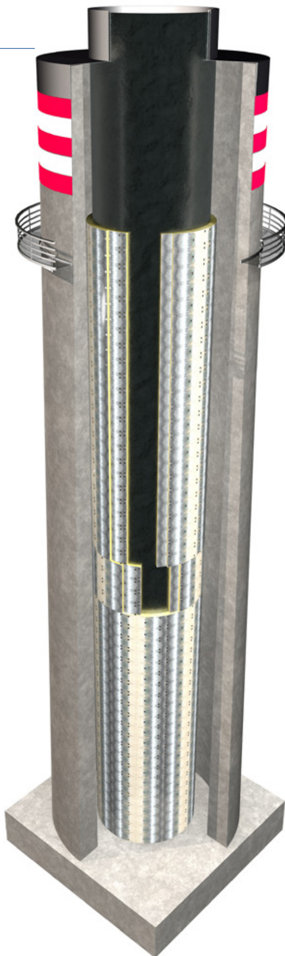
Figure 32. EXHAUST STACK
